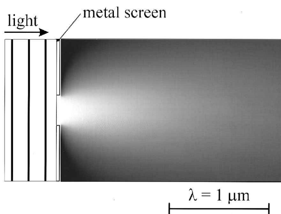
Figure 6. Lateral view (logarithmic intensity map) of the rapidly diverging light radiating from a subwavelength aperture. Note the confinement of the light near the aperture and the fast divergence at larger distances. Calculations were made using the Bethe–Bouwkamp approximation.
